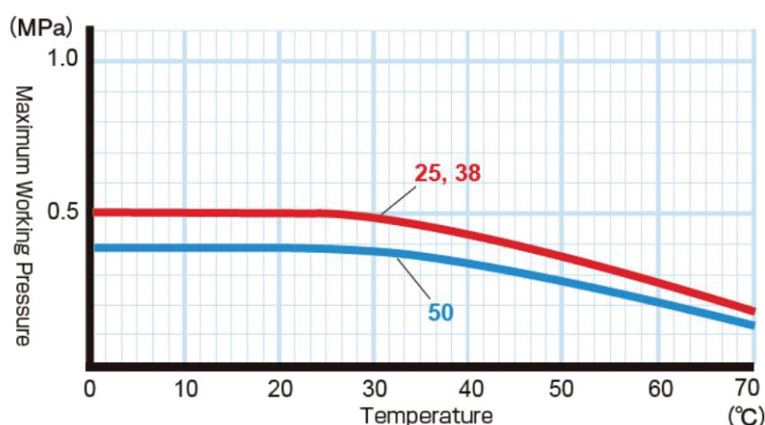
E-OHB: Relationship between Working Temperature and Maximum Working Pressure
